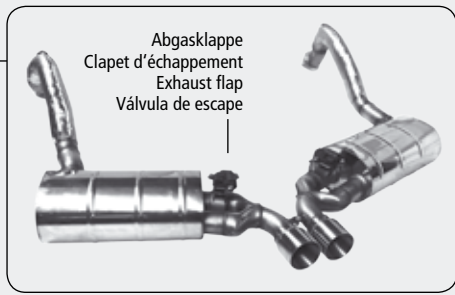
Double Central RACE Ø 90 mm
